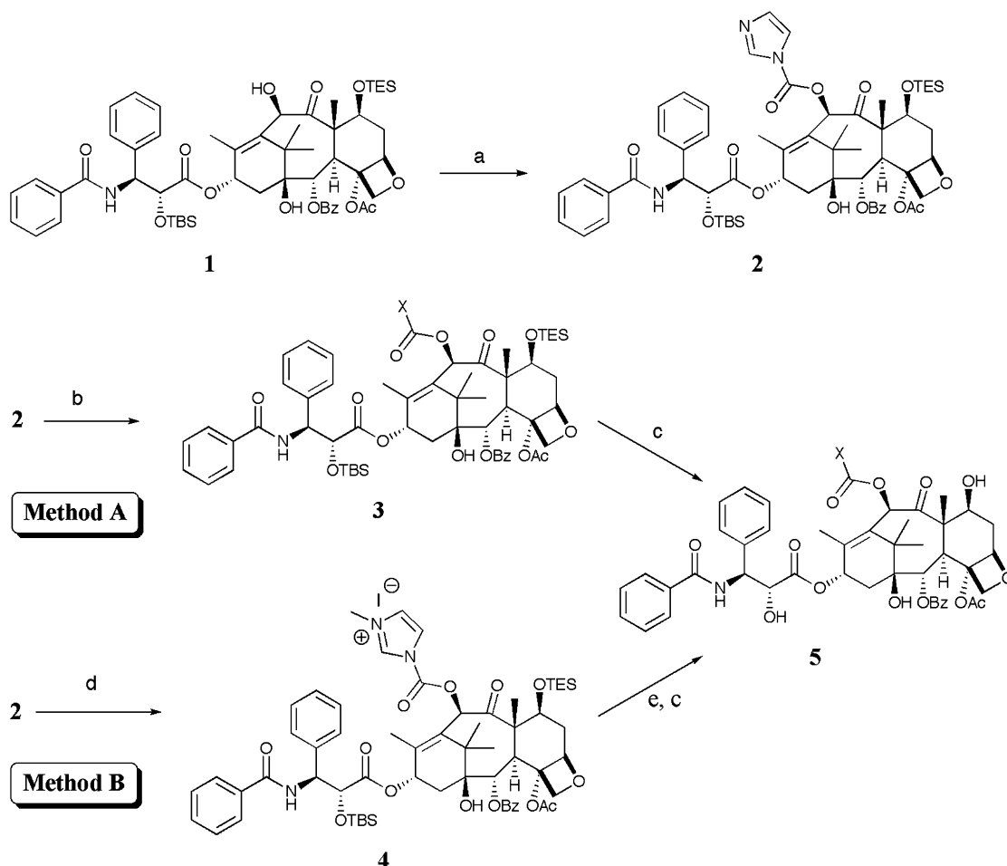
Figure 3. Reagents and conditions: (a) dichloromethane/carbonyl-diimidazole, rt, 16 h; (b) 5–7 equiv of amine in tert -butanol, 82 °C, 16 h; (c) acetonitrile/pyridine (1:1), HF/Py, 0 °C to rt, 4 h; (d) methyl iodide/acetonitrile, 55 °C, 3 h, (e) 2–3 equiv amine, rt.
