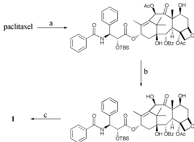
Figure 2. Reagents and conditions: (a) TBS-Cl, dimethylformamide, imidazole, 60 °C, 1.5 h; (b) hydrazine, ethanol, rt, 1.5 h; (c) TES-Cl, DMAP, dichloromethane, rt, 1 h.
